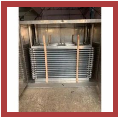
Vertical Plate Freezer
